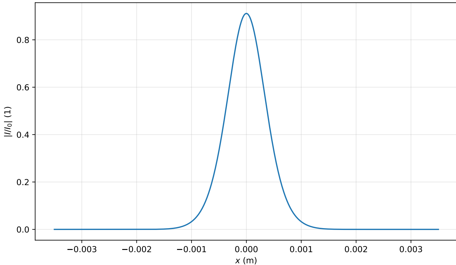
Intensity profile I(x, y = 0, z = 1.353m)/I_0 , P_{in}=0.4P_{cr} , artificial time
